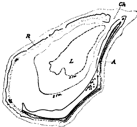
FIG. 172.—Plan of Minikoi Atoll in Laccadive Archipelago. A , the land elevated above the level of high-water mark; Ch , the boat channel; 5 fm , the five fathom line; 2 fm , the two fathom line; L , the lagoon with a maximum depth of 7 fathoms; R , the reef continuing the circle on the east side of the atoll, awash at high tides. (After Stanley Gardiner.)
